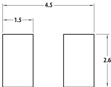
Figure 12: Recommended Soldering Pad Pattern
