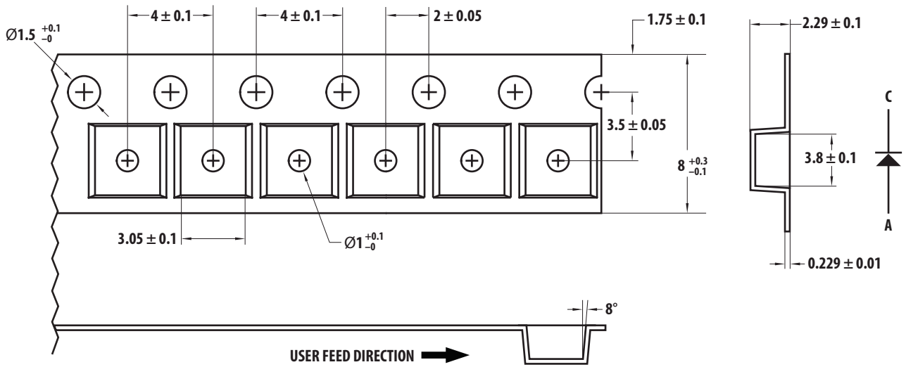
Figure 13: Carrier Tape Dimensions
