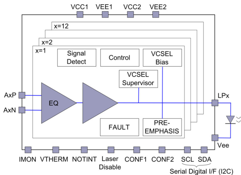
Figure 1: Device diagram
