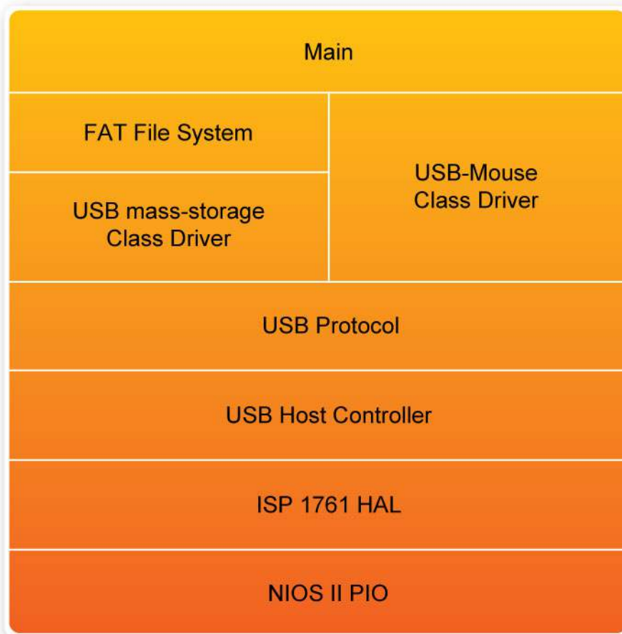
Figure 5.3. Software Stack of the USB-Host Demonstration
