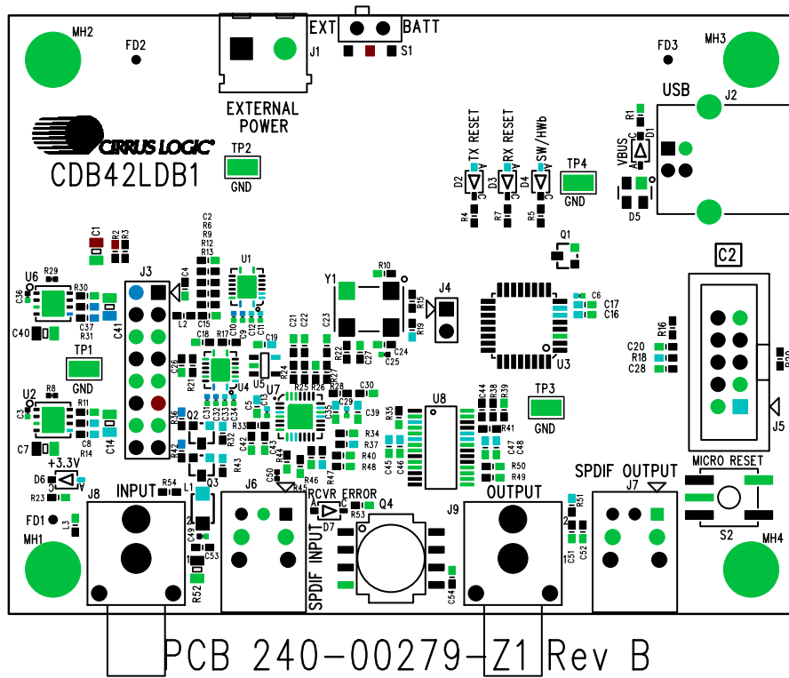
Figure 30. Silkscreen Top
