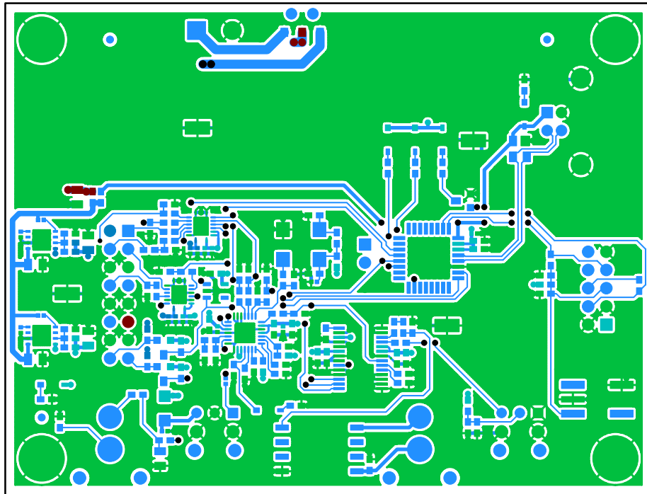
Figure 32. Top-Side Layer
