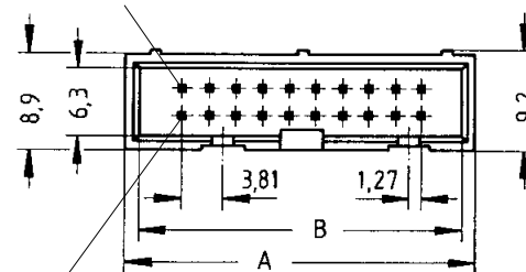
No. 1 contact
