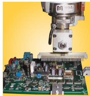
Pick-and-place machine for odd form components (Courtesy of JOT Automation GmbH)
