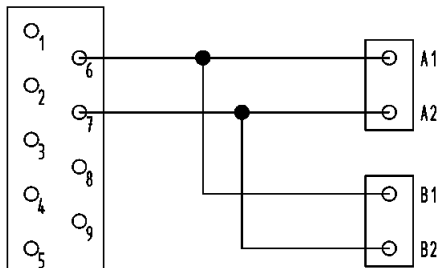
FIP interface
