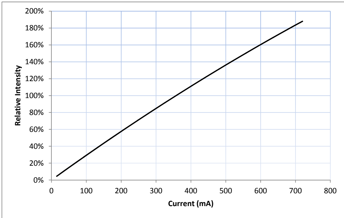
Figure 2: Typical Flux vs. Current, T_j = 25^\circ\text{C}
