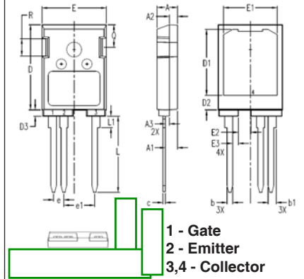
TO-247PLUS-HV Outline
