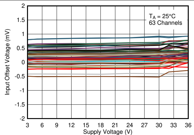
Figure 6-15. Input Offset Voltage vs. Supply Voltage at 25°C
