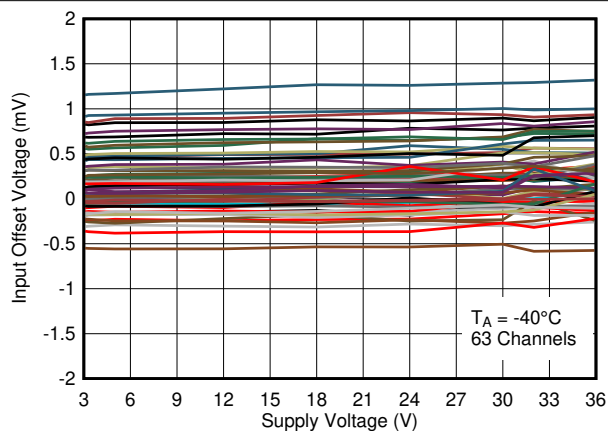
Figure 6-14. Input Offset Voltage vs. Supply Voltage at -40°C
