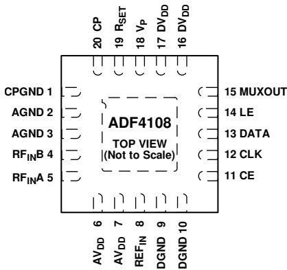
Figure 3. Pin Configuration
