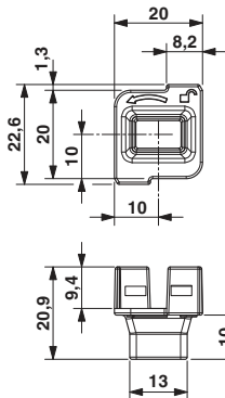
Sealing plug with locking for push-pull panel mounting frame
