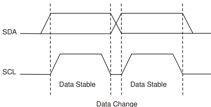
Figure 4-2. Data Transfer
