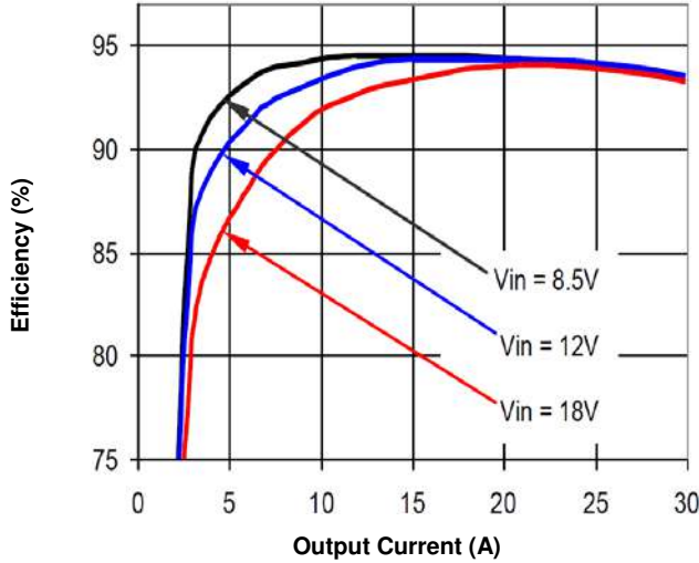
Figure 4a. Efficiency vs. Load Current (25°C)
