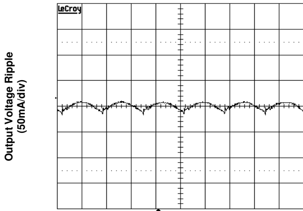
Time – t (2 \mu s/div) Figure 2c. Output Ripple Voltage ( V_{in}=12V , full load)
