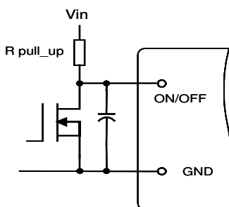
Figure 8. Circuit for Negative Logic Control
