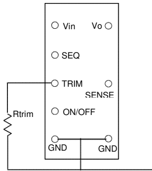
Figure 9. Circuit for Output Voltage Trim
