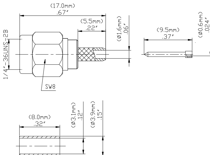
Model 72946 SMA PLUG STRAIGHT CRIMP, RG174, 188, 316
