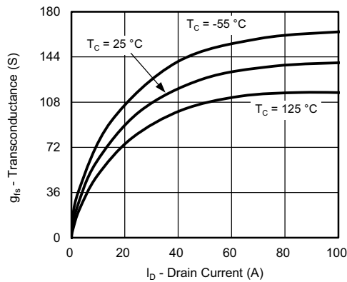
Transconductance
