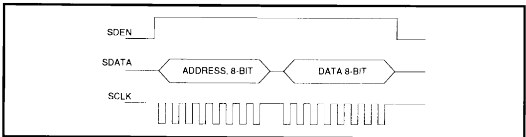
FIGURE 2: Serial Port Data Transfer Format
