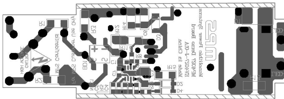
Figure 3 - Bottom Layer
