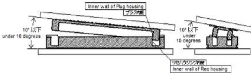
△ 図-2 内壁合せによる挿抜 Figure-2 Mating aligning to inner wall of housings (Acceptable)
