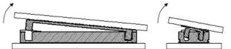
× 図-5 こじり抜去 Figure-5 Withdrawal with twisting the connector at an angle (Not Good)
