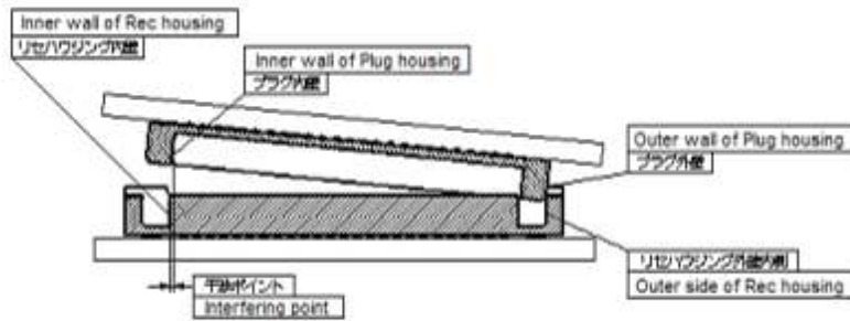
× 図-3 外壁合せによる挿抜 Figure-3 Mating aligning to outer wall of housings (Not Good)
