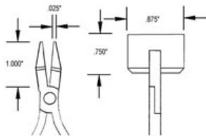
508-US Straightening Pliers with Metal Jaws
