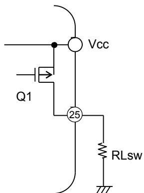
Figure 6 High-side Switch
