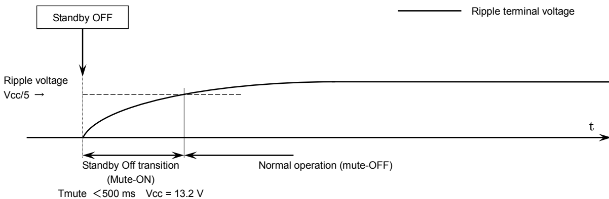
Figure 5 standby-Off Mute
