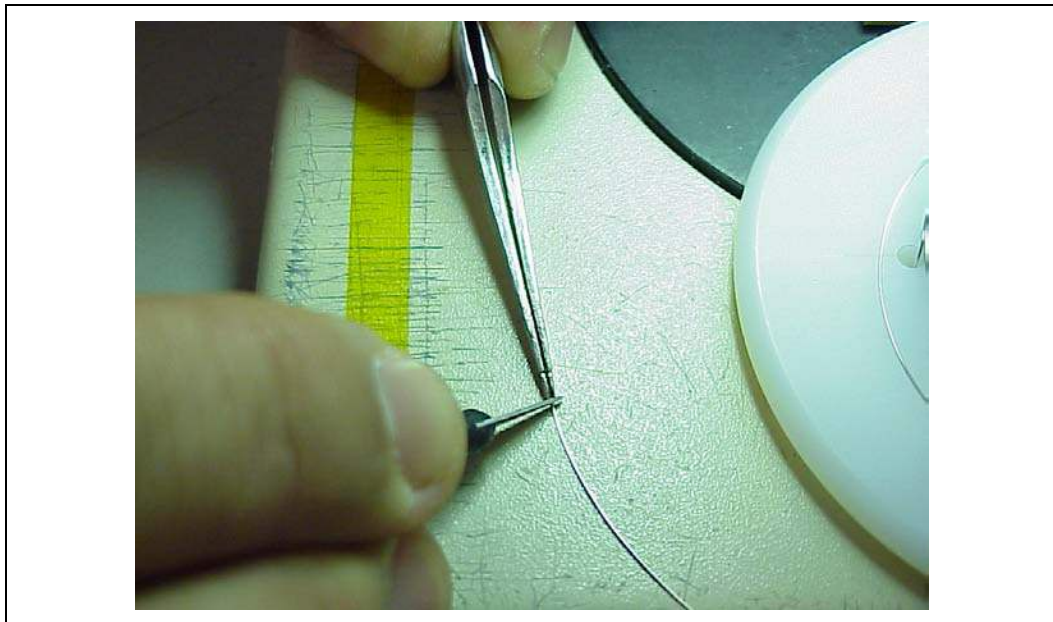
Figure 7-25. Cutting Solder
