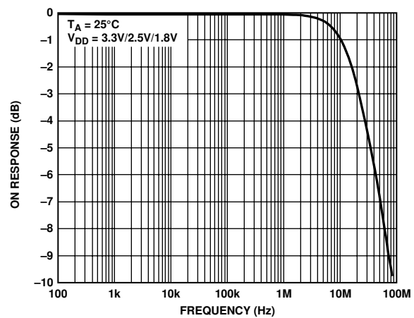
Figure 14. Bandwidth
