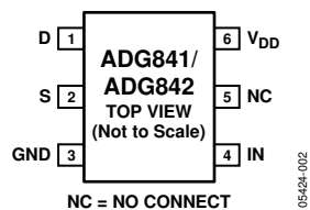
Figure 2. 6-Lead SC70
