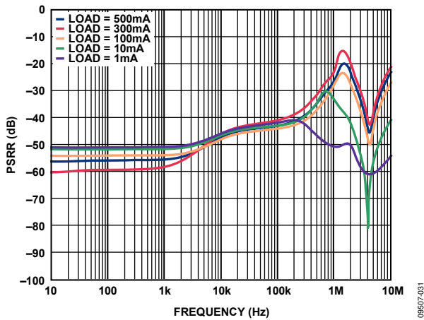
Figure 36. Power Supply Rejection Ratio vs. Frequency, V_{OUT} = 3.3 V , V_{IN} = 3.8 V
