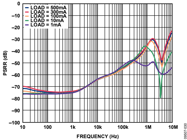
Figure 35. Power Supply Rejection Ratio vs. Frequency, V_{OUT} = 3.3 V , V_{IN} = 4.3 V
