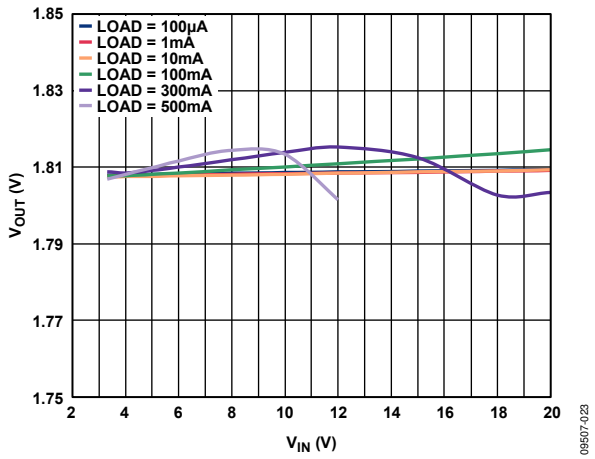
Figure 25. Output Voltage vs. Input Voltage, V_{OUT} = 1.8 V
