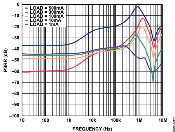
Figure 40. Power Supply Rejection Ratio vs. Frequency, V_{OUT} = 5 V , V_{IN} = 5.3 V
