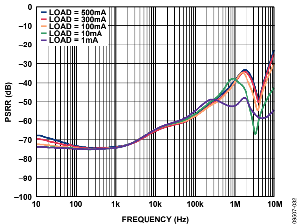
Figure 37. Power Supply Rejection Ratio vs. Frequency, V_{OUT} = 5 V , V_{IN} = 6.5 V
