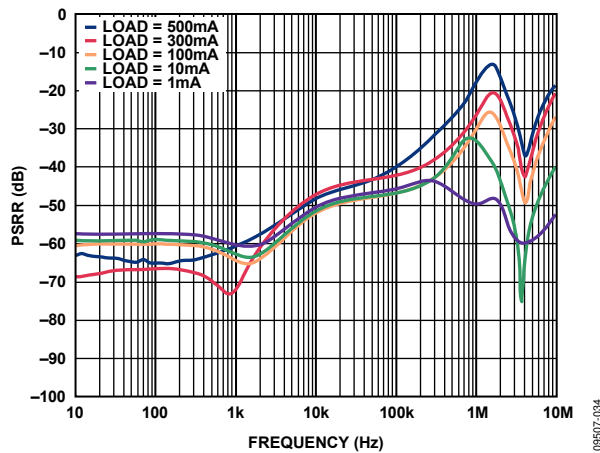
Figure 39. Power Supply Rejection Ratio vs. Frequency, V_{OUT} = 5 V , V_{IN} = 5.5 V
