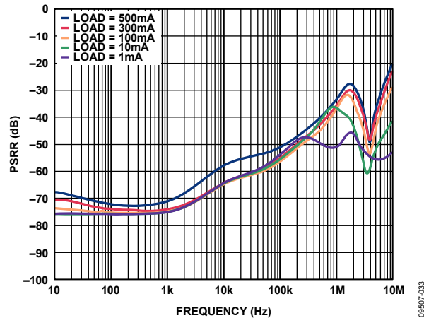
Figure 38. Power Supply Rejection Ratio vs. Frequency, V_{OUT} = 5 V , V_{IN} = 6 V
