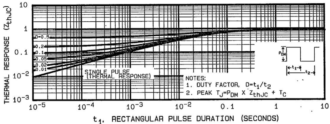
Fig. 16 - Maximum Effective Transient Thermal Impedance, Junction-to-Case vs. Pulse Duration
