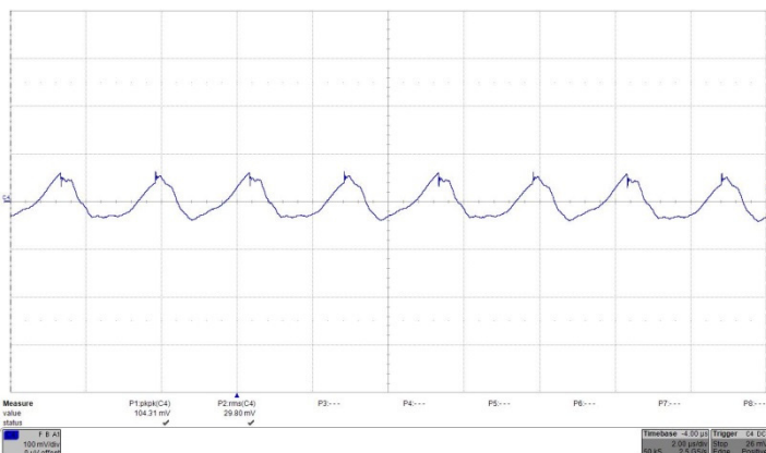
Fig. 37: Output voltage ripple (100 mV/div.) at full rated load current into a resistive load at Vin = 24 V. Co = 2 x 470 μF/70mΩ. Time: 2 μs/div.
