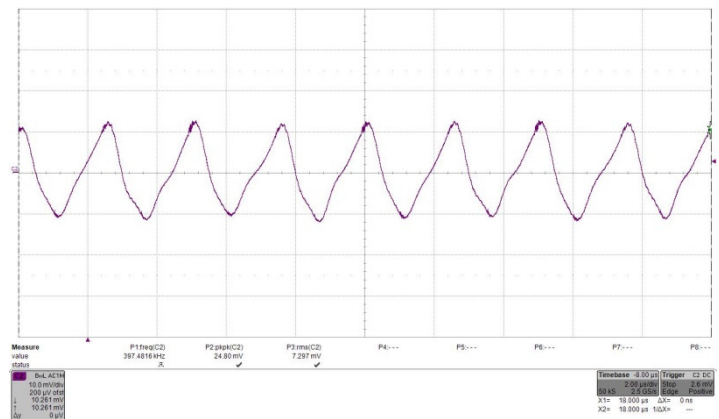
Fig. 38: Input reflected ripple current, ic (500mA/mV), measured at input terminals at full rated load current at Vin = 24 V. Refer to Fig. 2 for test setup. Time: 2 μs/div. RMS input ripple current is 7.3*0.5A = 3.65A rms .
