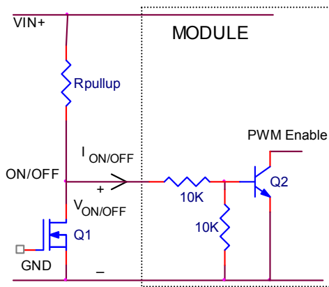
Figure 44. Circuit configuration for using negative On/Off logic.
