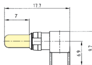
Premating contact
