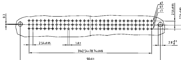
Panel cutout
