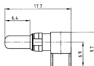
Plug contact
