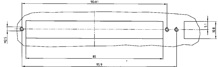
Panel cutout
