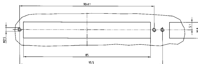
Panel cutout
