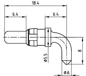
Plug contact
