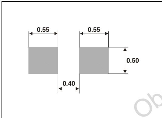
Figure 24. Footprint
