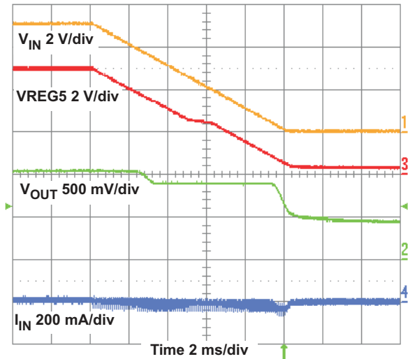
Figure 4-9. TPS54427 Shut-down Relative to V_{IN}
