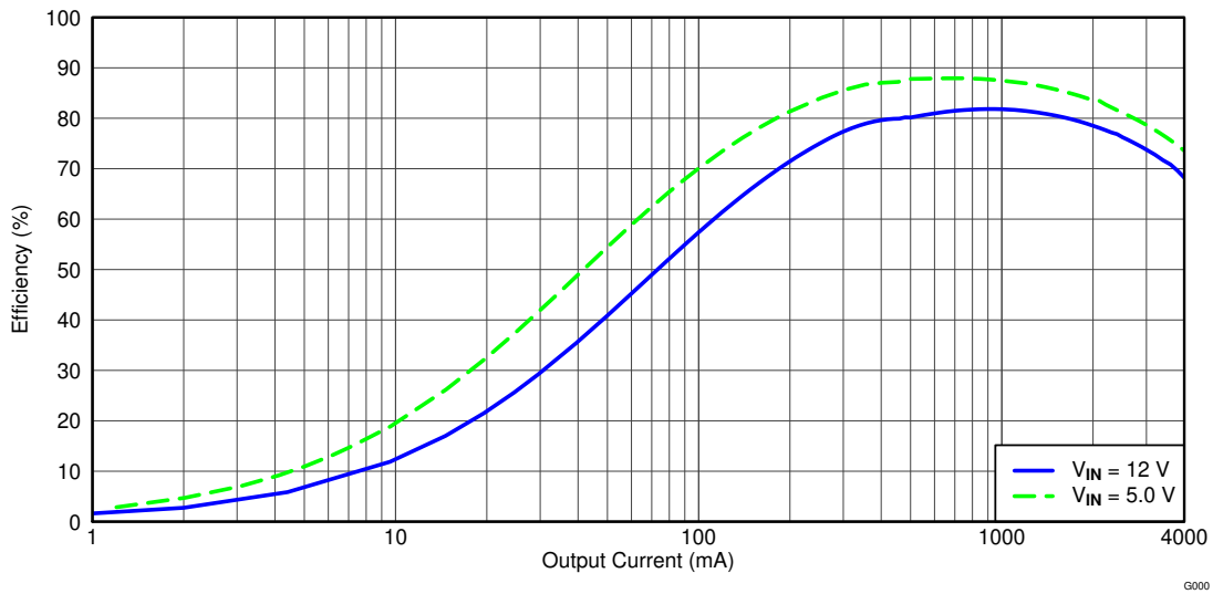
Figure 4-2. TPS54427 Light-Load Efficiency
