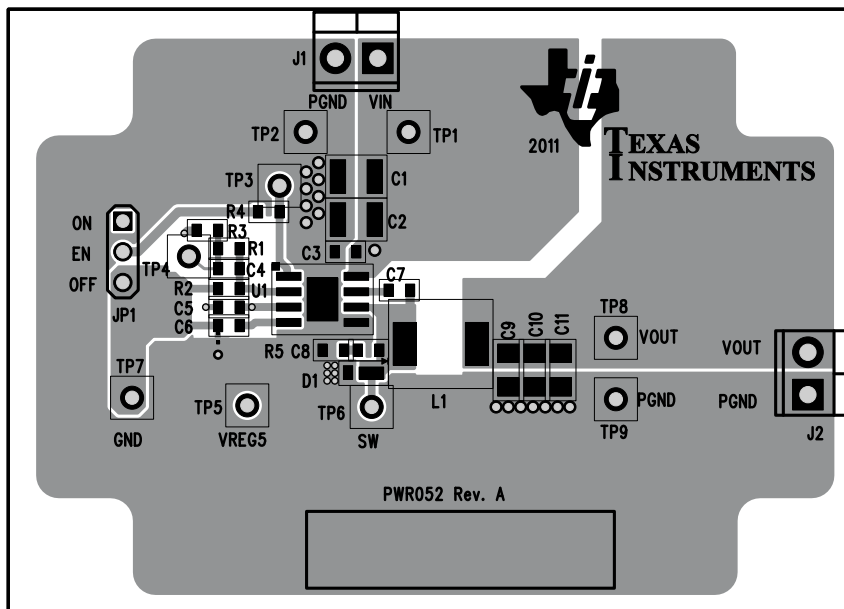
Figure 5-1. Top Assembly
