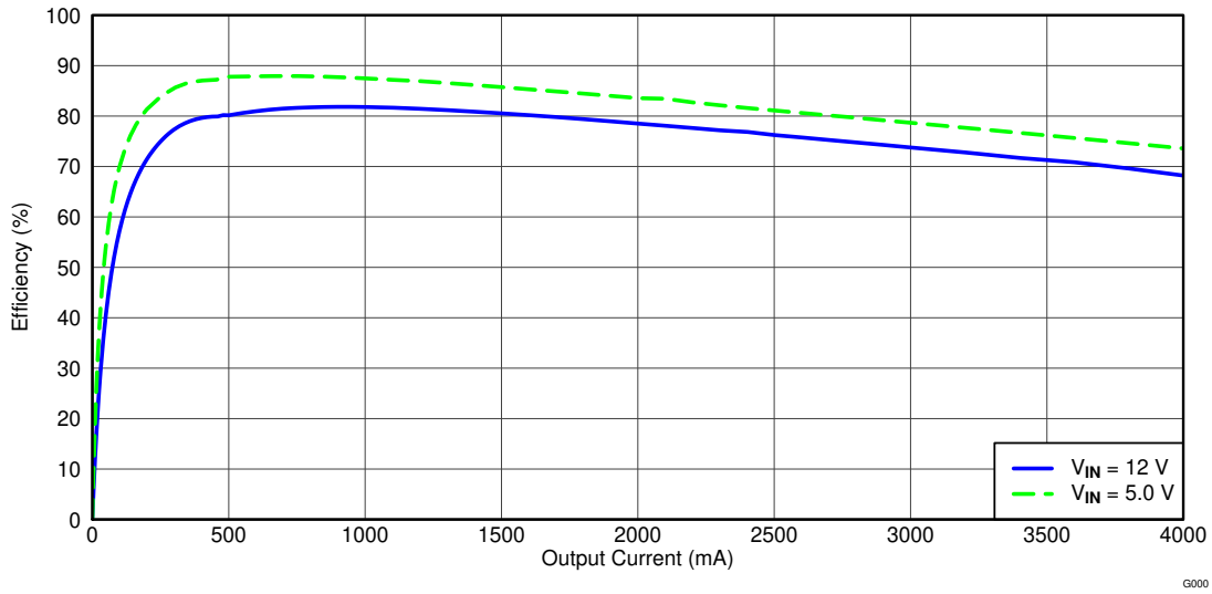
Figure 4-1. TPS54427 Efficiency
