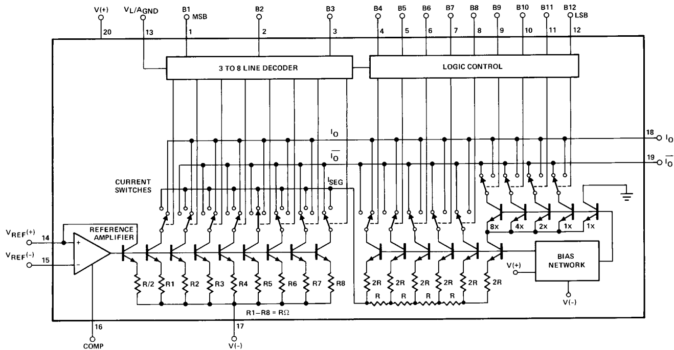
Simplified Schematic
