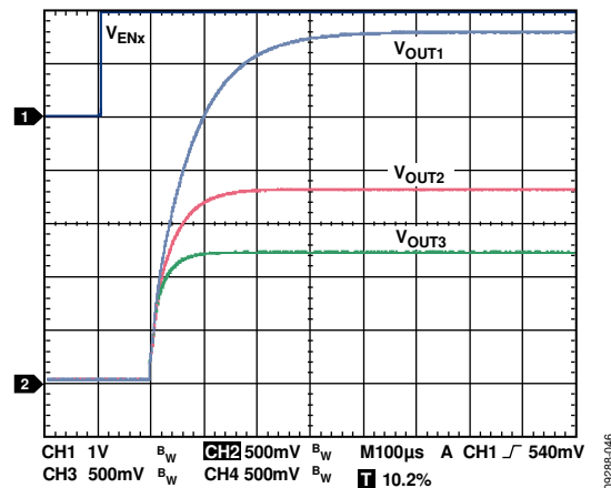
Figure 55. Typical Start-Up Time, I_{LOAD1} = I_{LOAD2} = I_{LOAD3} = 100\ \text{mA} , CH1 = V_{ENx} (the Enable Voltage), CH2 = V_{OUT1} , CH3 = V_{OUT2} , CH4 = V_{OUT3}
