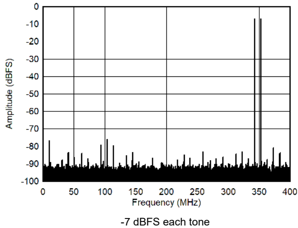
Figure 7-51. Dual Tone FFT at 348 MHz -7 dBFS each tone
