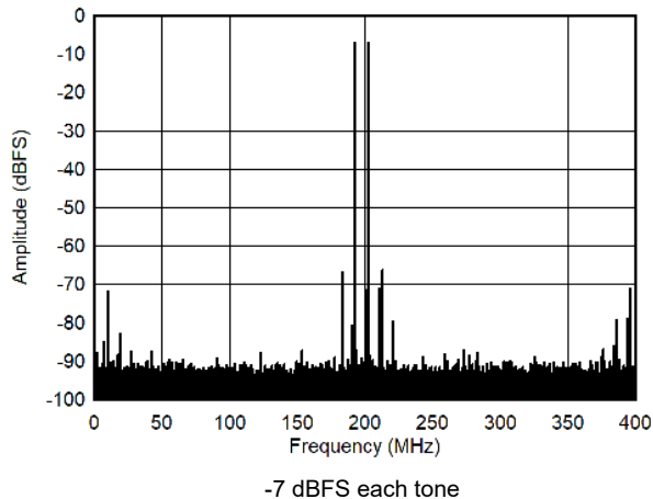
Figure 7-53. Dual Tone FFT at 1798 MHz -7 dBFS each tone
