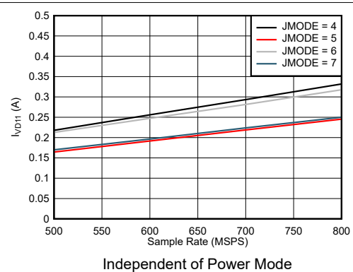
Figure 7-78. Quad Channel, I_{VD11} vs F_S for JMODES 4 - 7
