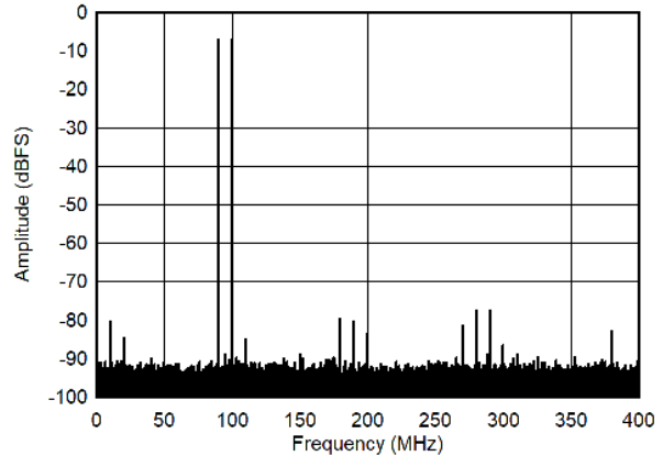
Figure 7-50. Dual Tone FFT at 95 MHz -7 dBFS each tone
