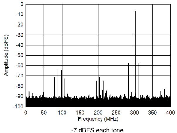
Figure 7-54. Dual Tone FFT at 2698 MHz -7 dBFS each tone
