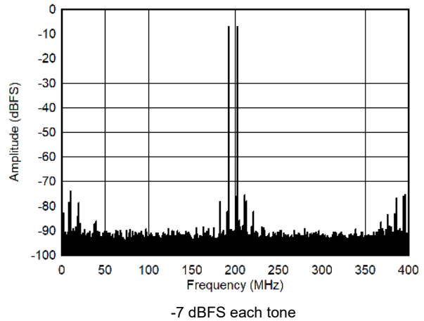
Figure 7-52. Dual Tone FFT at 998 MHz -7 dBFS each tone
