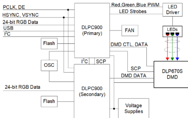
DLP670S Simplified Schematic
