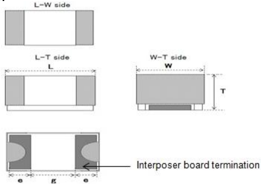
image:Dimension
