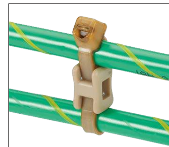
Longer spacing with one cable tie, parallel
