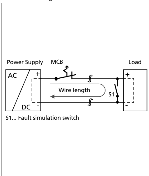
Fig. 26-9 Test circuit
