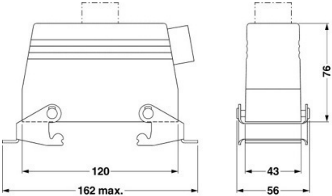
Dimensioned drawing
