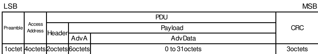
Figure 1. Bluetooth® Low Energy Advertising Channel packet format
