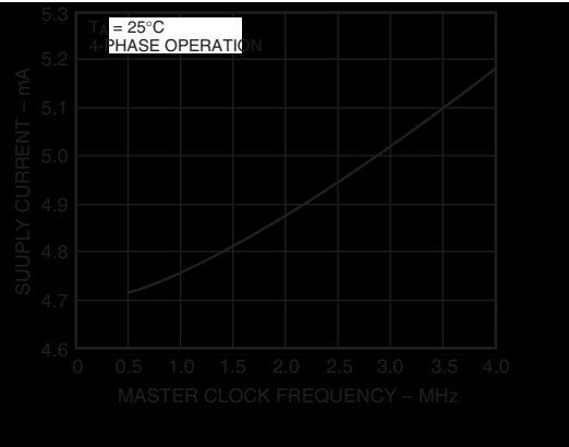
TPC 2. Supply Current vs. Master Clock Frequency
