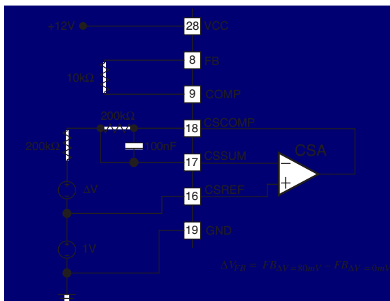
Test Circuit 2 – Voltage Positioning
