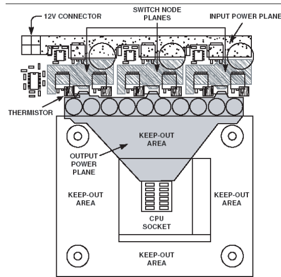
Figure 11. Layout Recommendations
