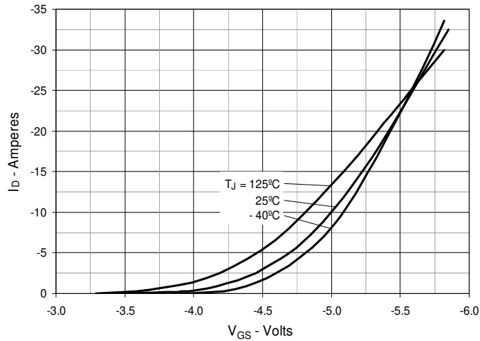
Fig. 7. Input Admittance
