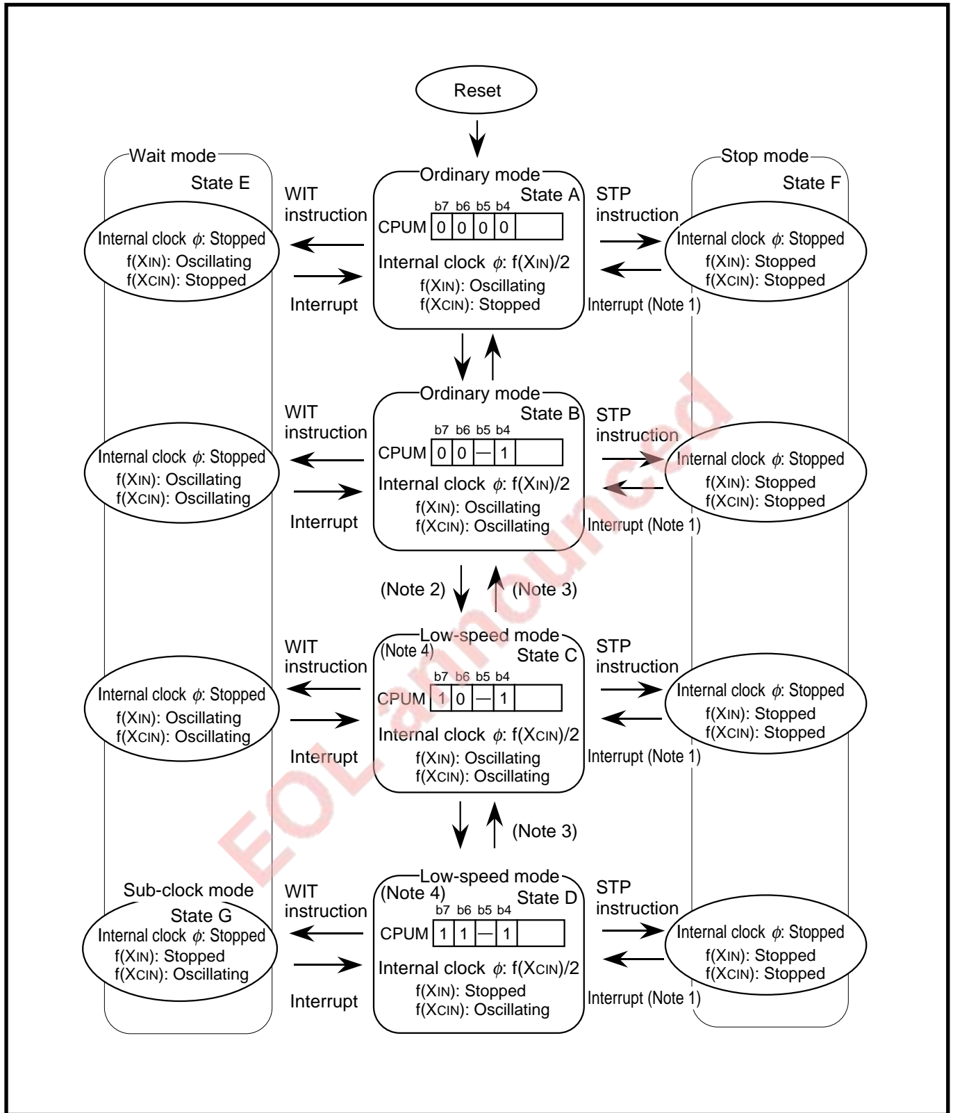
Fig. 1.18.1 State transitions
