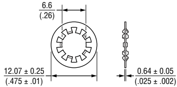
LOCKWASHER H-37-2
