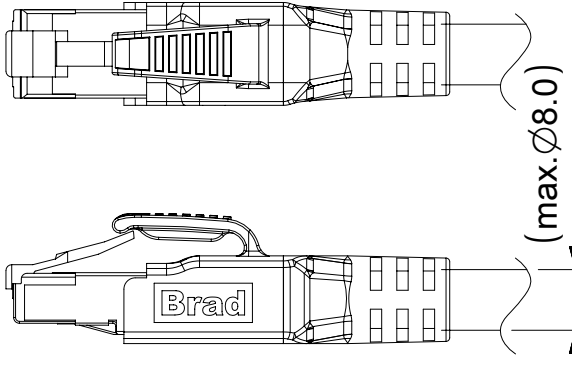
OVERMOLD VIEW FOR CABLES O.D.≥6.7mm
