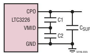
Figure 3. Charging a Single Supercapacitor
