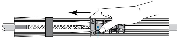
Snap Tool Installation
