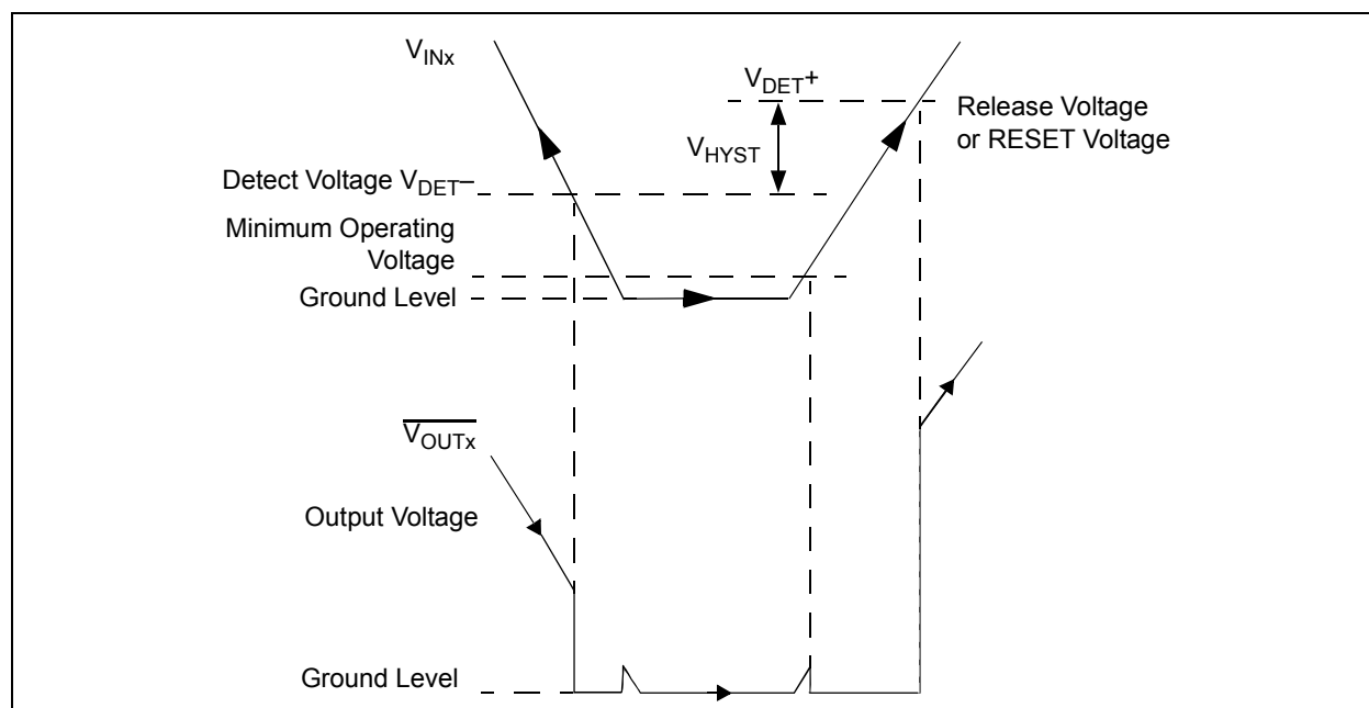
FIGURE 3-1: Timing Diagram.
