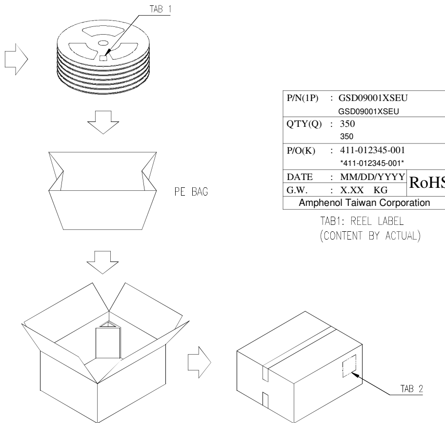
PACKING OPERATION DIAGRAM
