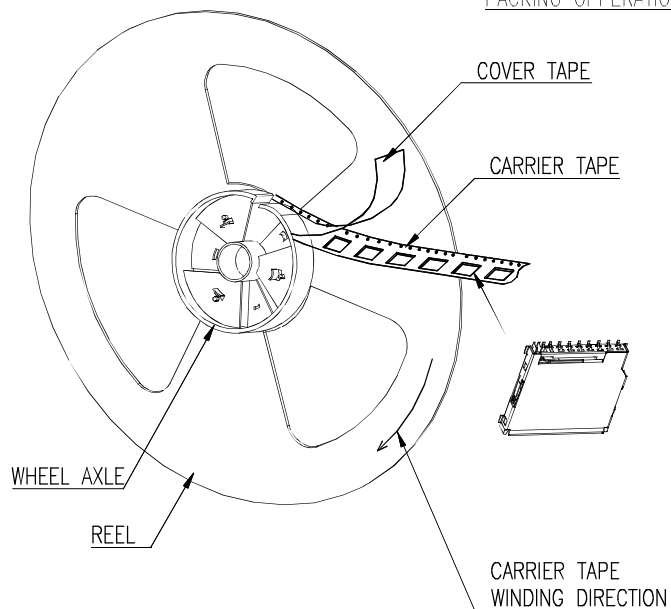
PACKING OPERATION DIAGRAM
