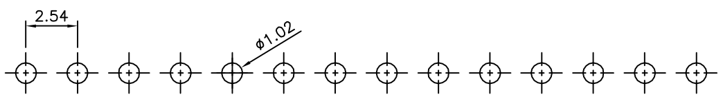
Recommended P.C.B Layout(Top Side) (PCB Board Tolerance±0.05)
