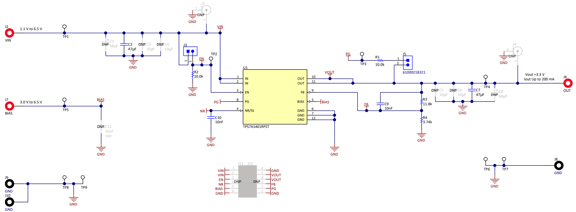
Figure 6. TPS7A54EVM-031 Schematic
