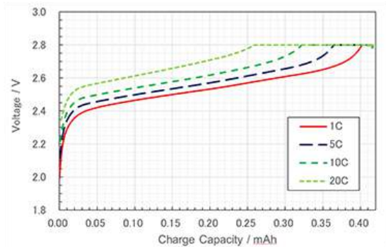
Charge characteristics
