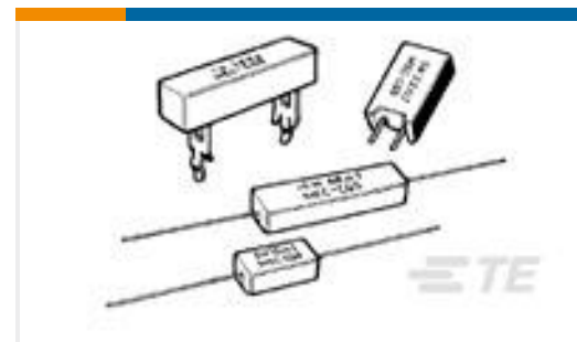
TE Part #1623785-7 SQM10 75R 5% (WIRE)
